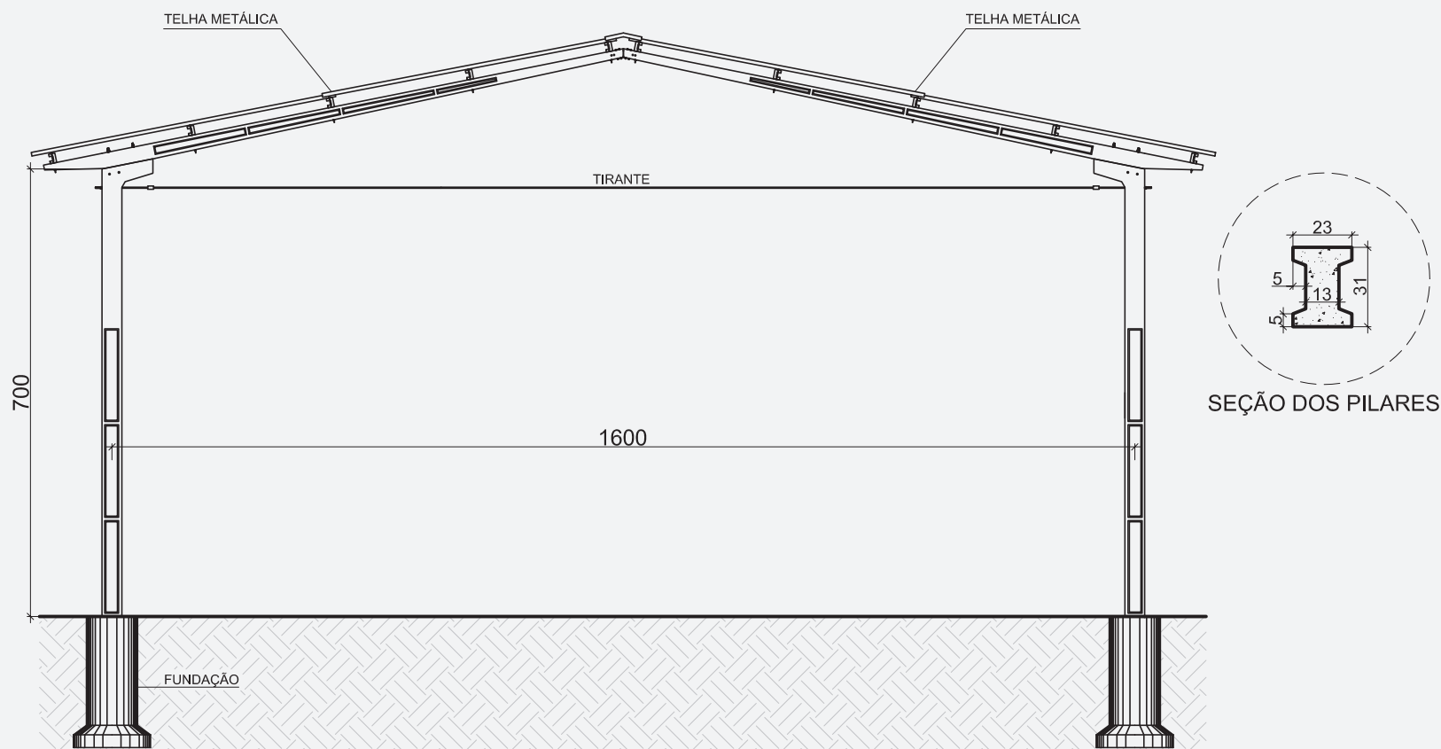
Vista Frontal
